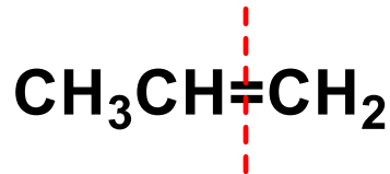
propen
