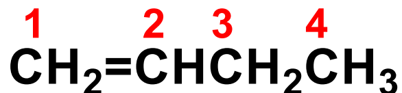
1-buten
