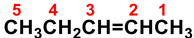
2-penten
