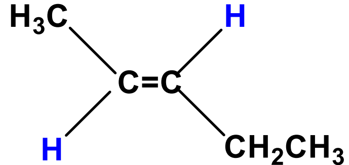
trans -2-penten
