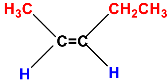
2-penten
